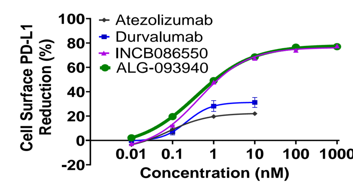
Figure 1: Effect of ALG-093940 vs. INCB086550 and FDA-approved PD-L1 antibodies on PD-L1 cell surface expression
